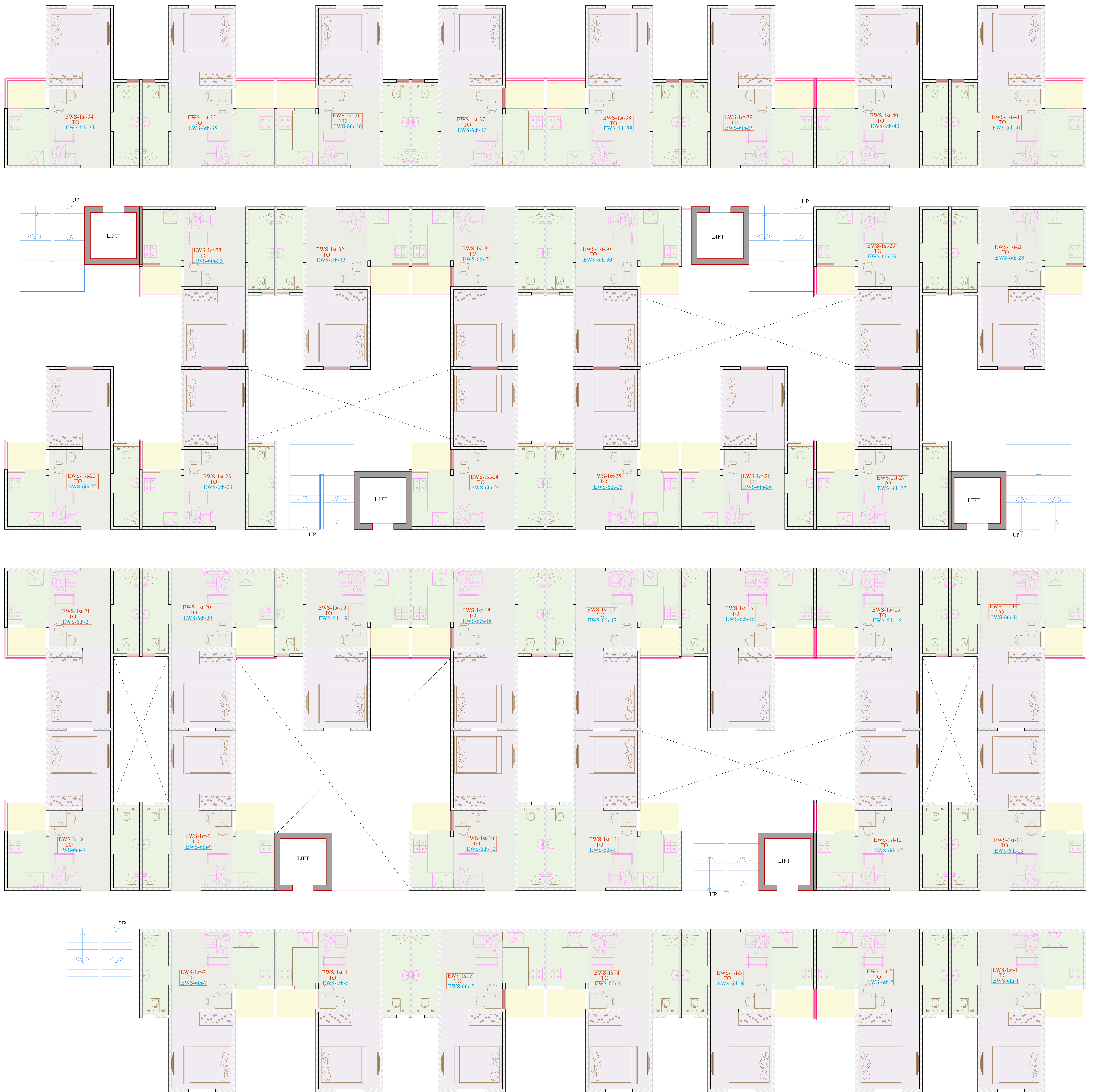
TYPICAL FLOOR PLAN (BLOCK-E)
